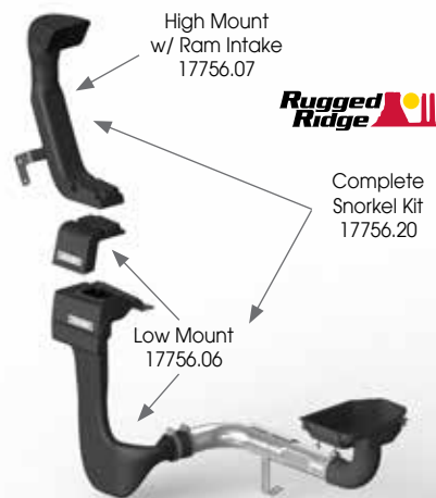
HIGH MOUNT W/ RAM INTAKE
